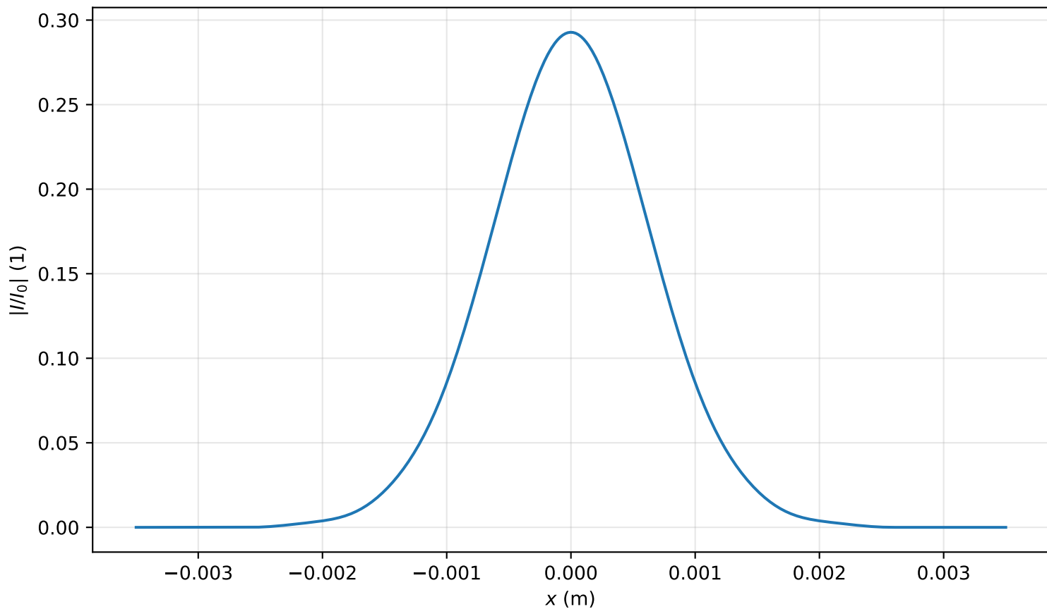
Intensity profile I(x, y = 0, z = 3.901m)/I_0 , P_{in}=0.3P_{cr} , artificial time
